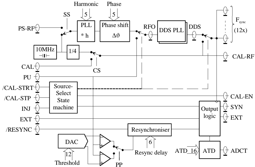
Fig. 1 Block-diagram of the VME RF-MUX and Synchroniser
