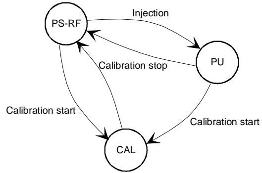
Fig. 2 The RF-MUX state machine
