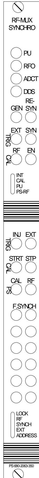
Fig. 3 Front panel
