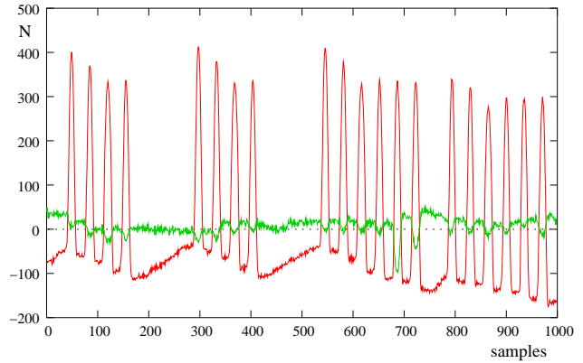
Fig 2: Example of PU signals: LHC beam at 2nd batch injection. \Sigma and \Delta_x .
