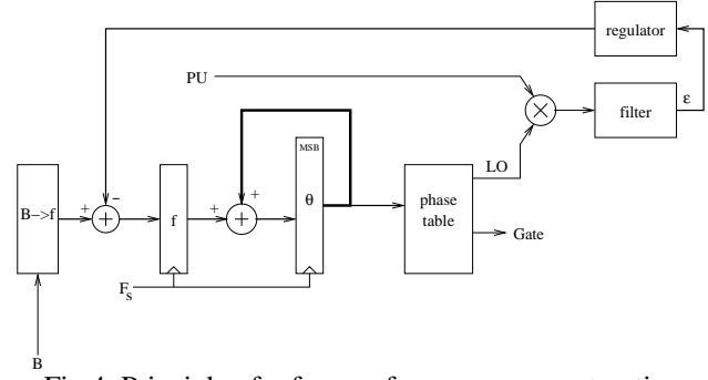
Fig 4: Principle of reference frequency reconstruction
