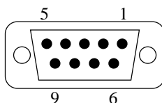
Figure 12: The layout of the V.24 interface
