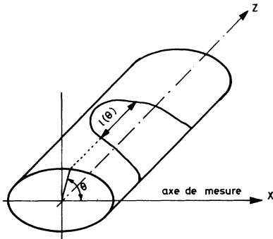
Fig. 1 : Co-ordinate system.
