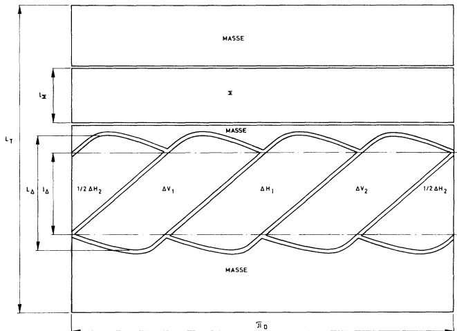
Fig. 3 : Development of a pick-up electrode
