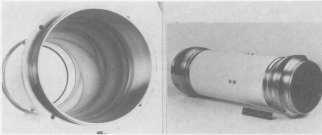
Fig. 4 : Inside of a pick-up electrode Fig. 5 : Pick-up electrode shown without shielding
