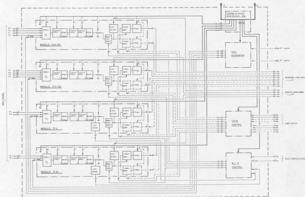
Fig. 6 : Station arrangement
